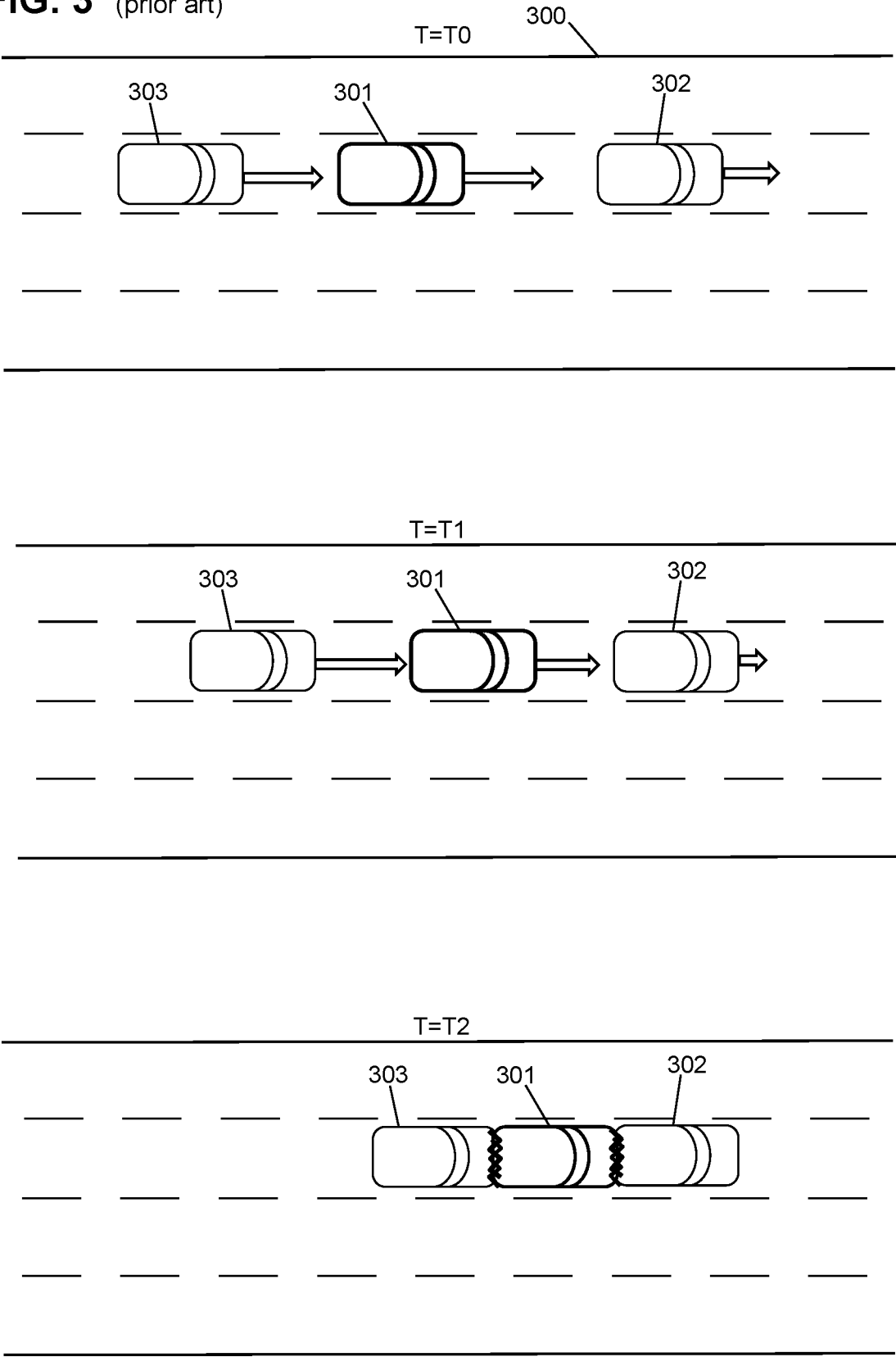
FIG. 3 (prior art)
